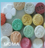
MDMA
